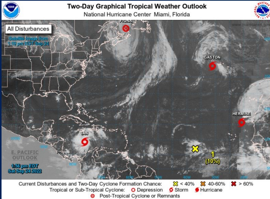
Fuente: National Oceanic and Atmospheric Administration NOAA, 2022
