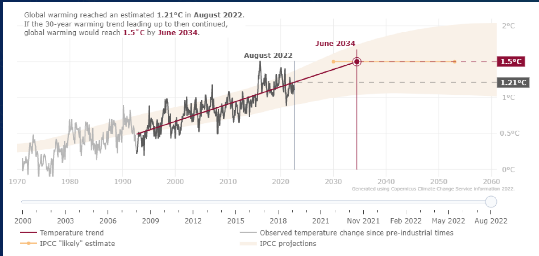
Fuente: Copernicus Climate Change Service information 2022
